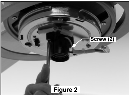
Fig-2. Install Down Light Socket Assembly with two screws provided.
