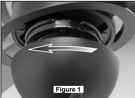
Fig-1. Remove Lower Cover Assembly by twisting in a counter-clockwise direction.
