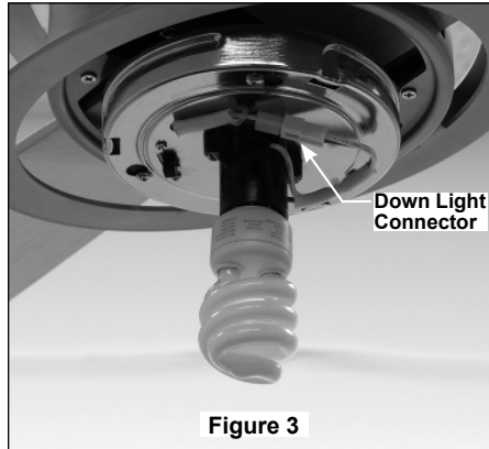
Fig-3. Securely attach the two-pin Down Light connector to wiring harness socket on the Switch Cup Assembly and the 13 watt CFL bulb provided.
